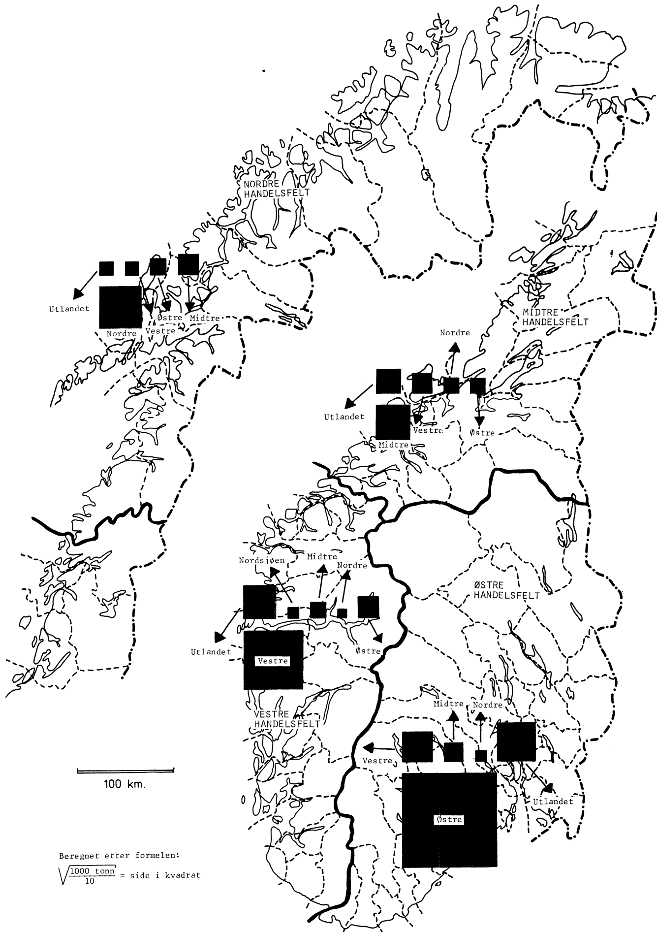
Figur 4. Transportmengde mellom handelsfelt. Alle skip 25 - 3 000 bruttotonn. 1975 Tonnage carried between trade regions. All vessels 25 - 3 000 gross tons. 1975
